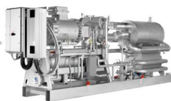
SABROE ComPAC chillers, 200-2200 kW
